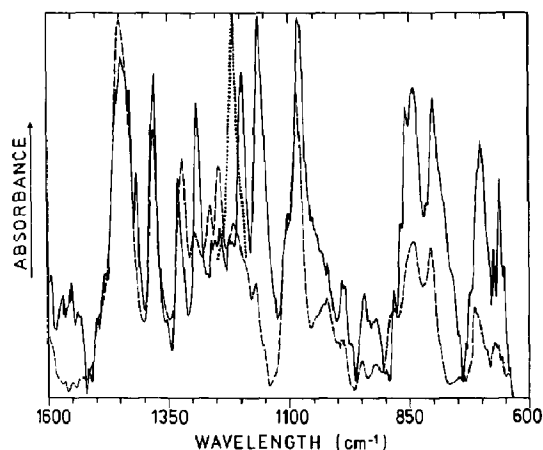
Fig. 5. FTIR absorption spectra of PQ-3-PQH 2 -3 mixture before (—) and after (---) precooling in the range 1600–600 \text{cm}^{-1} and a fragment of PQH 2 -3 spectrum (.....) in the \nu(\text{C-O}) region.
